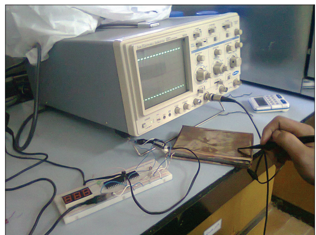
Figure 1: Experimental design used for electrical stimulation. Electric fields (20 mv/cm, 1 kHz) are delivered to the cultured cells
