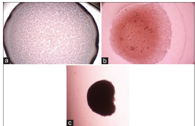
Figure 3: Representative invert microscopy images of micromass droplet in electric field applied group. (a) 1 st day. (b) 2 nd day. (c) 3 rd day. Magnification \times 20
