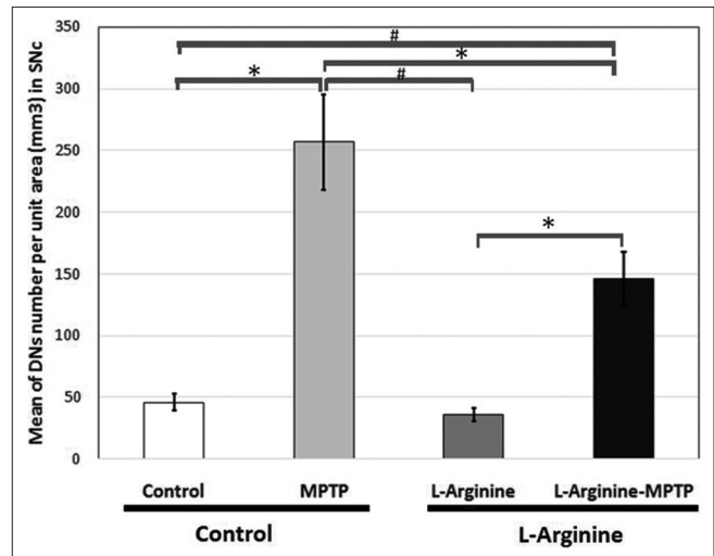
Figure 2: * P < 0.05 ; significant difference. # P < 0.01 ; significant difference. Graph 1: Mean of dark neuron numbers per unit area (mm 3 ) in the substantia nigra pars compacta subdivision of Balb/c mice and its comparison in the different studied groups. The data show that the mean number of dark neurons per unit area in methyl-4-phenyl-1,2,3,6-tetrahydropyridine group significantly increased in substantia nigra pars compacta comparing to L-arginine and control Balb/c mice. Evaluation of therapeutic effects on dark neuron production in substantia nigra pars compacta subregion revealed a significant reduction in the mean number of dark neurons in L-arginine - methyl-4-phenyl-1,2,3,6-tetrahydropyridine group. Data present in mean \pm standard error of the mean
